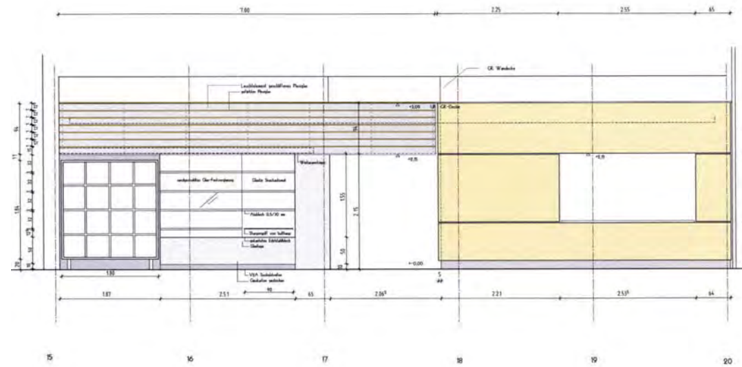
Wandabwicklung Cafeteria
